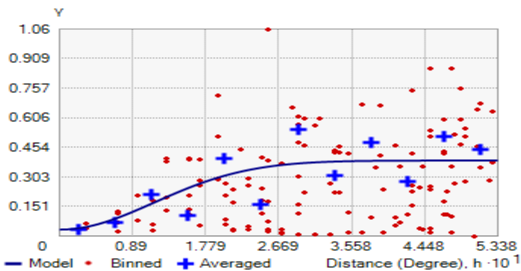
Figure 3. Semivariogram of Soil Organic Carbon
